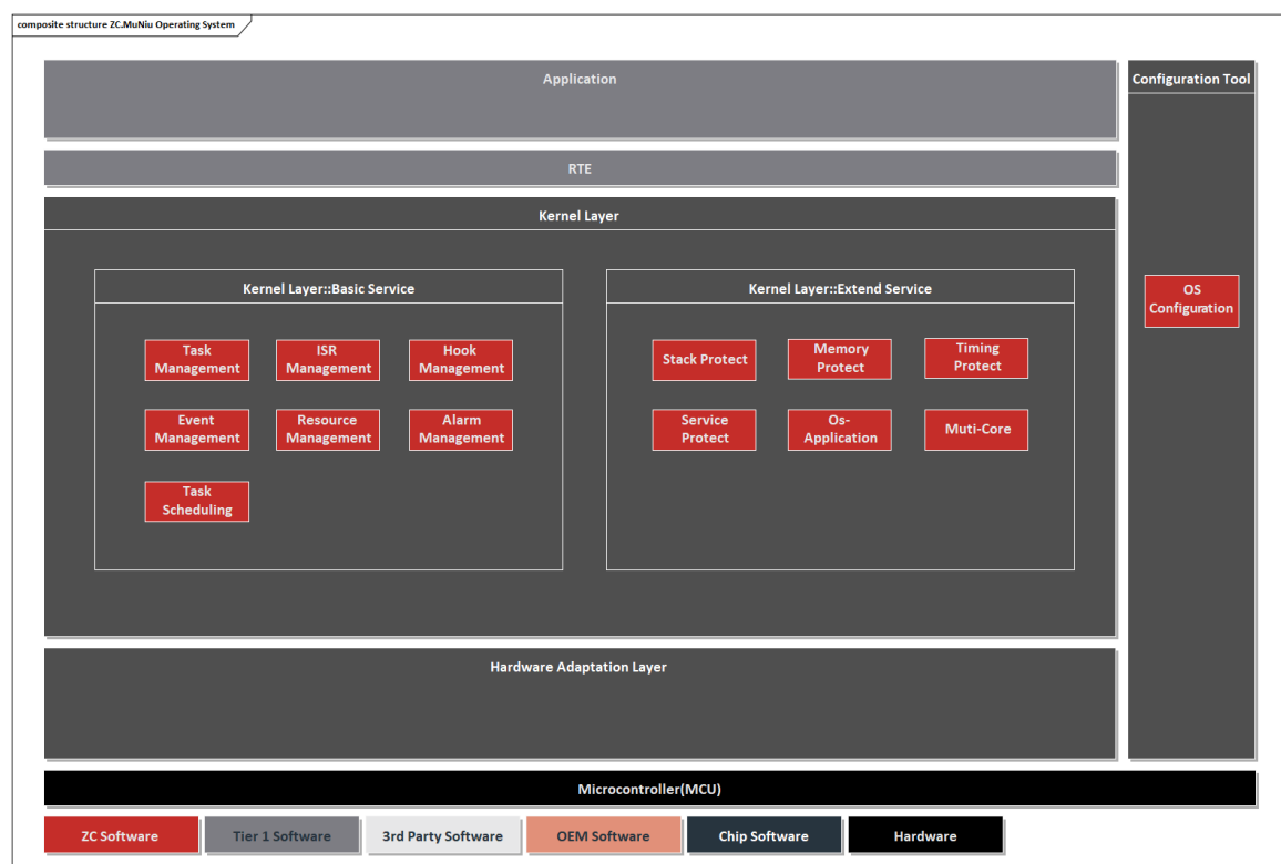
知从木牛操作系统 OS 产品软件架构 ZC.MUNIU OPERATING SYSTEM SOFTWARE ARCHITECTURE
