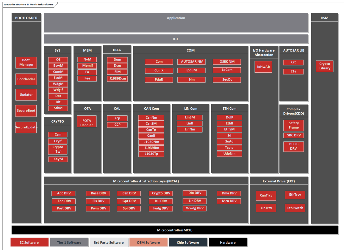
知从木牛基础软件架构 ZC.MUNIU BASIC SOFTWARE ARCHITECTURE
